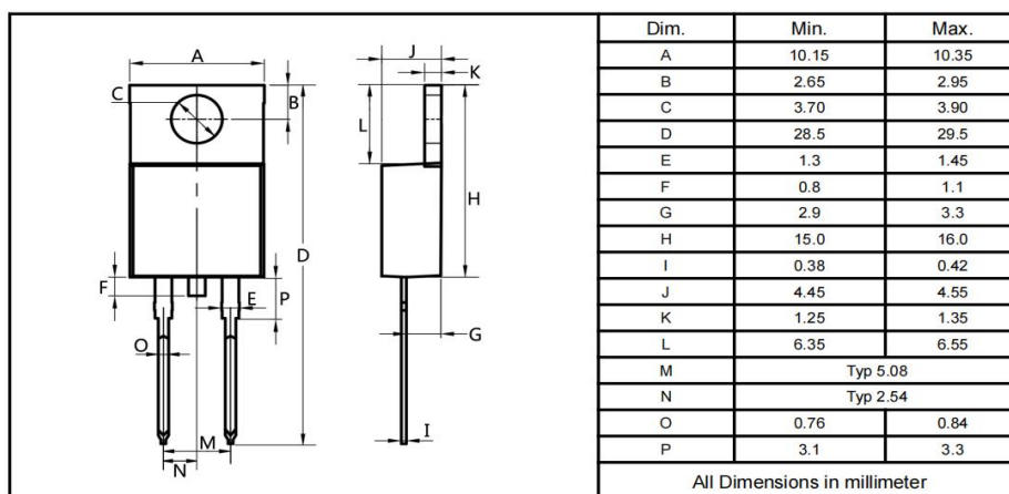
TO-220FAC
